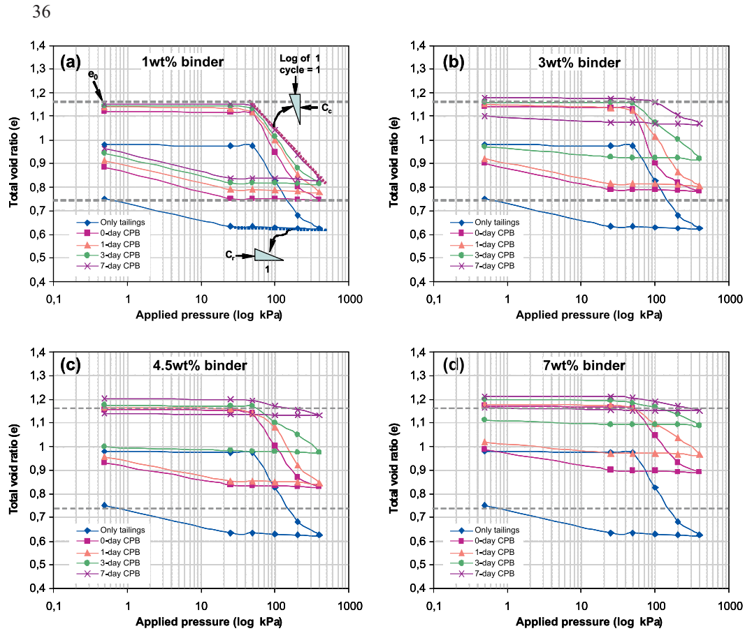
Fig. 2. Consolidation curves of CPB samples a – 1 wt%, b – 3 wt%, c – 4.5 wt%, d – 7 wt% binder
