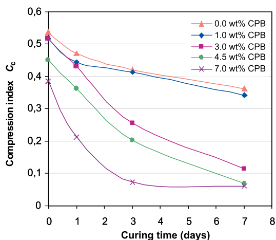
Fig. 3. Compression index vs. curing time
