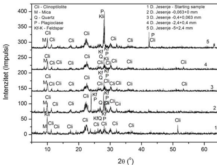
Fig. 2. Powder diffractogram of Donje Jesenje samples
