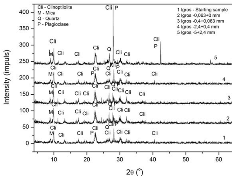
Fig. 1. Powder diffractogram of Igroš samples
