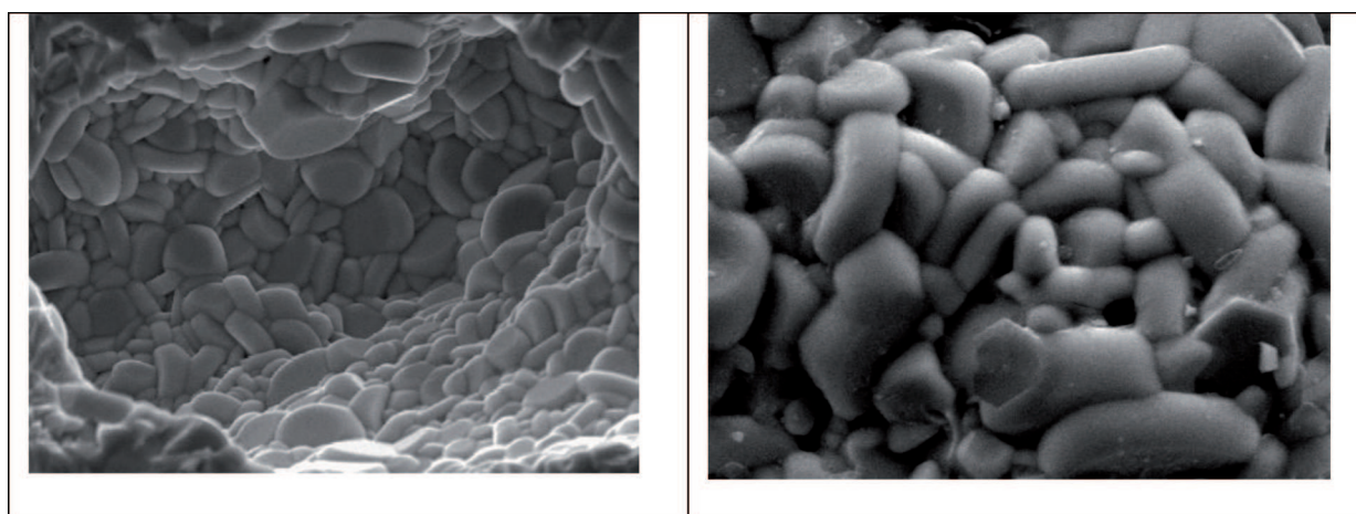
Fig. 1. SEM images of pure [2] and doped BaBi 2 Nb 2 O 9 ceramics
