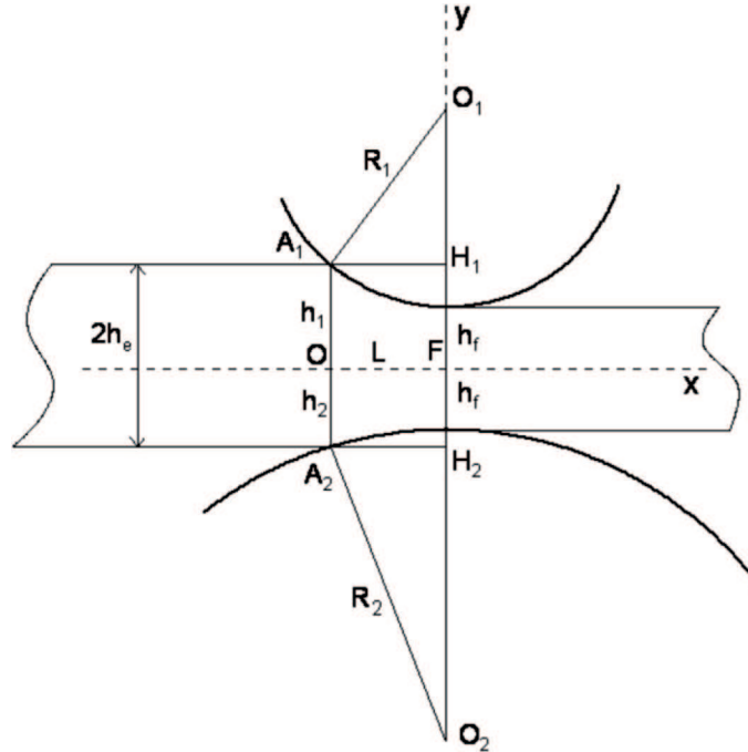
Fig. A1. Schematic representation of ASR including the definition of the various geometrical parameters
