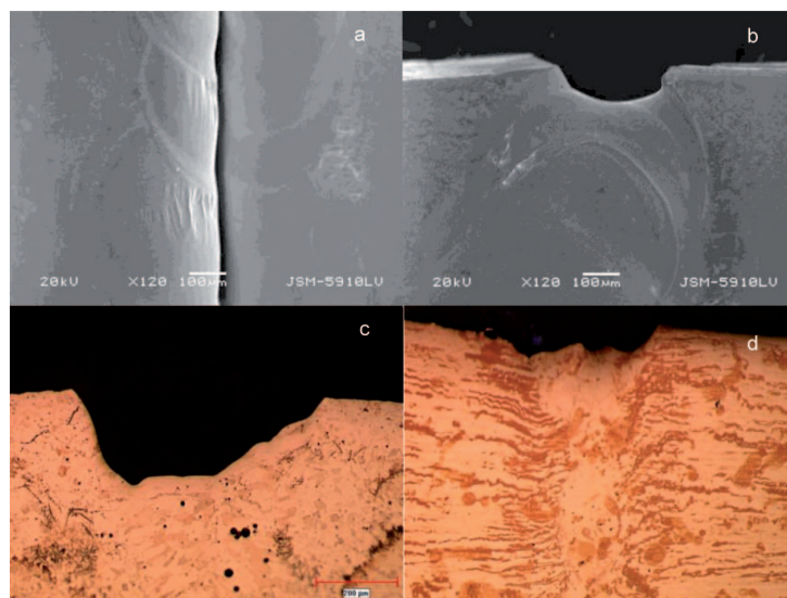
Fig. 11. 14 ct red micrographs: a) workpiece 2 b) workpiece 5 c) workpiece 6 d) workpiece 3
