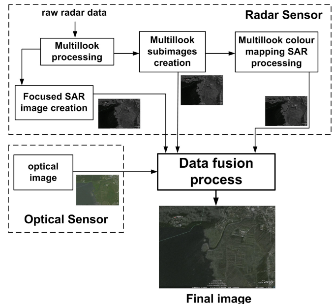
Fig. 1. Block diagram of the radar and optical images fusion algorithm.
