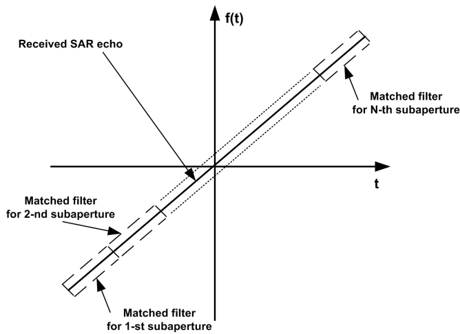
Fig. 2. Received SAR echo with marked sub-apertures matched filters.
