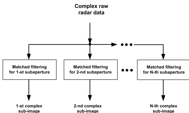
Fig. 3. Simplified block diagram of the multilook processing.
