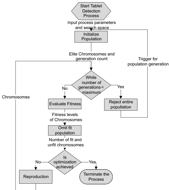
Fig. 2. Flow diagram of the proposed algorithm.
