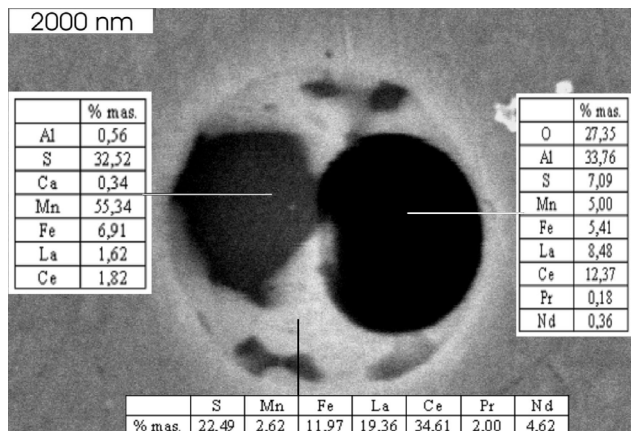
Fig. 15. Microanalysis of selected elements in the spherical particles of non metallic inclusions in modified cast steels. SEM, EDS. Composition contrast
