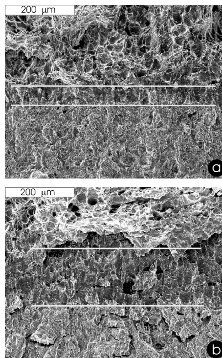
Fig. 4. Strength zones at non-modified (a) and modified (b) SEM
