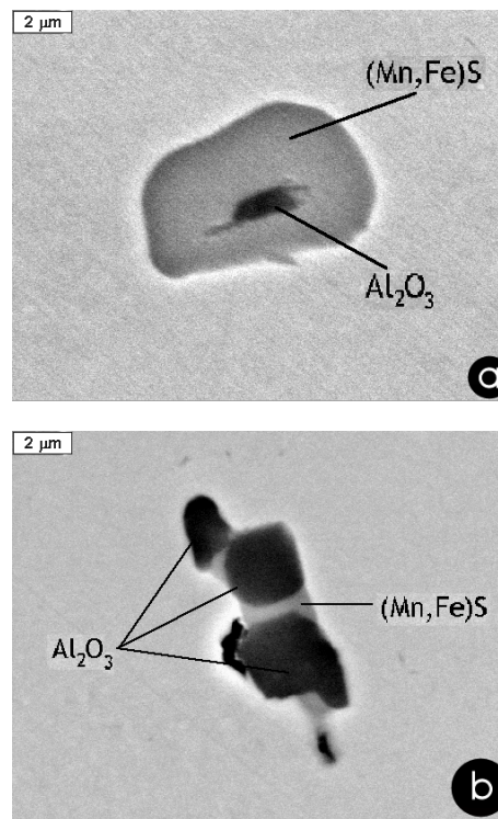
Fig. 11. Non metallic inclusions in non modified cast steels. Non etched. SEM. Composition contrast
