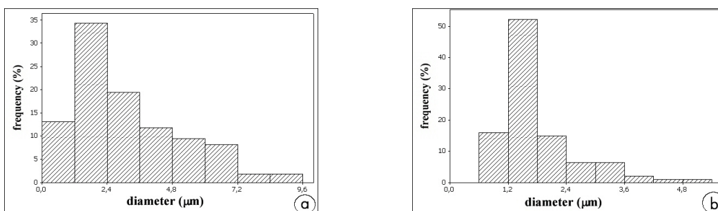
Fig. 10. The bar charts for the non-metallic inclusions diameters for the GP240GH cast steel: a – non modified and b – modified
