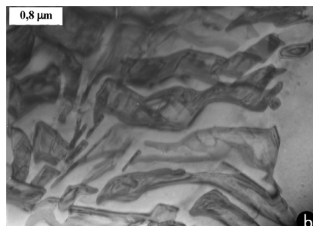
Fig. 8. The cementite plate configurations for the GP240GH cast steel perlite (a) – non modified and (b) – modified. TEM a thin film
