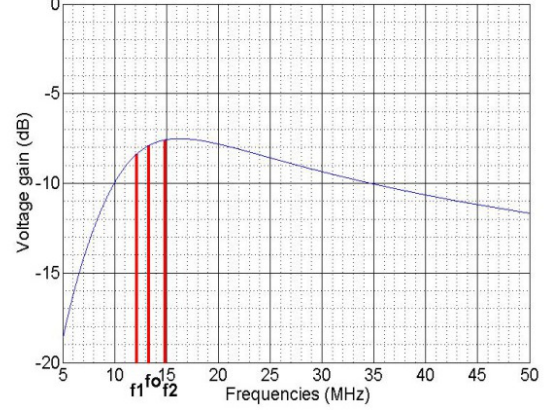
Voltage gain versus splitting and traditional resonant frequencies(N=2)
