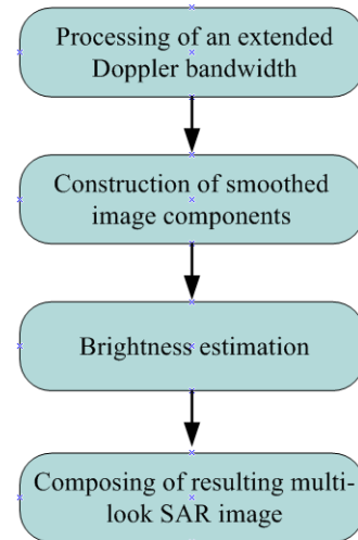
Fig. 6. Range-Doppler processing with extended number of looks for radiometric error correction.
