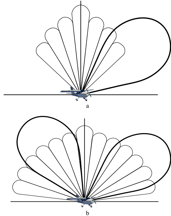
Fig. 4. Real antenna beam and synthetic beams (a – common multi-look processing, b – extended number of looks)
