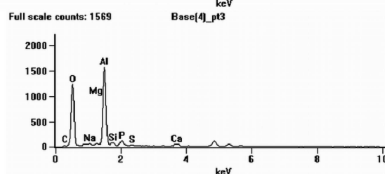
Fig. 9. X-ray energy spectra (EDS) from selected areas for sample No 4 of catalytic converter carrier which was wrongly used (overheated or poisoned)
