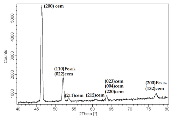
Fig. 3. Diffractometer trace for area A (Fig. 1)
