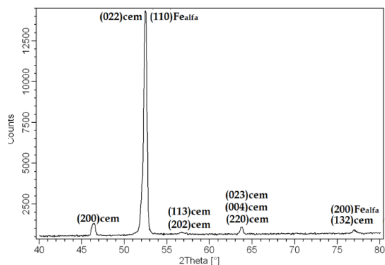
Fig. 5. Diffractometer trace for area B diagonally (B2) to the axis of the sample (Fig. 1)
