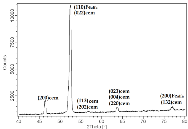
Fig. 7. Diffractometer trace for area C (Fig. 1)
