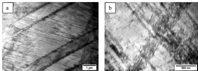
Fig. 4. TEM micrographs of the Fe-28Mn-9Al-1C steel after 23% reduction and ageing at 550°C for 2 hours (BF)
