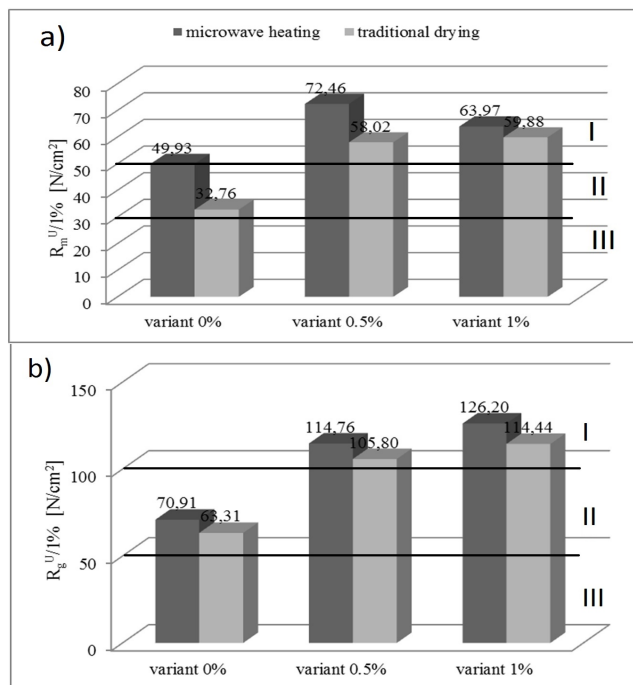
Fig. 1. Quality indices acc. to strength criteria: a) R_m^U and b) R_g^U per 1 wt% of binder 137 for sandmixes hardened by physical methods
