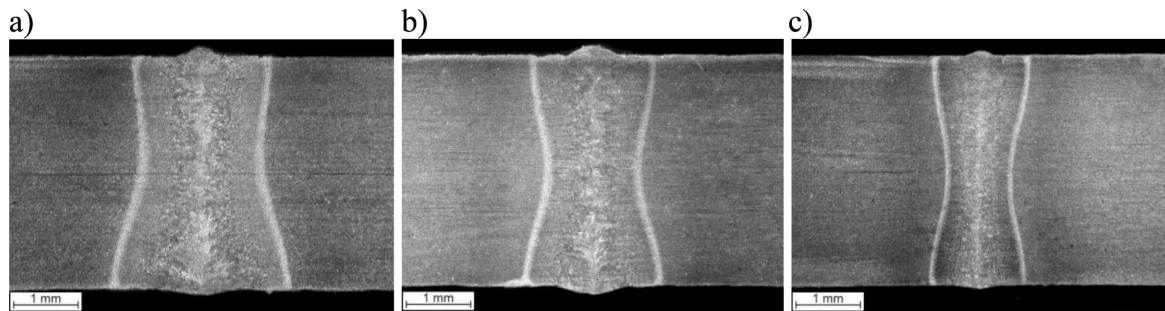
Fig. 2. Macrographs of the cross-section of bead-on-plate welds produced at laser power of 3300 W and different welding speeds: a) 2.0 m/min; b) 4.0 m/min; c) 6.0 m/min (Table 2)
