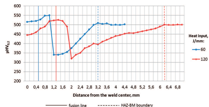
Fig. 9. Microhardness distribution on the cross section of the butt joints
