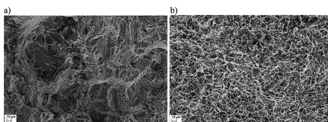
Fig. 11. SEM micrographs of fracture surface after bending tests of the joints welded at the heat input of: a) 60 J/mm; b) 120 J/mm (magnification 2500x)
