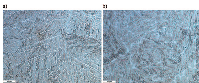
Fig. 8. Microstructure of the center region in the weld metal of butt joints welded at heat input of: a) 60 J/mm; b) 120 J/mm
