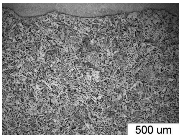
Fig. 2. High amount of acicular ferrite in weld (71%) after Ar/CO 2 micro-jet cooling
