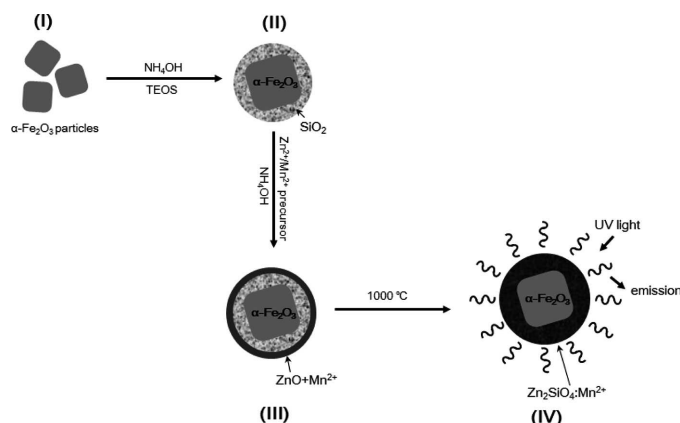
Fig. 1. Schematic diagram is synthetic \alpha\text{-Fe}_2\text{O}_3@Zn_2\text{SiO}_4:\text{Mn}^{2+}
