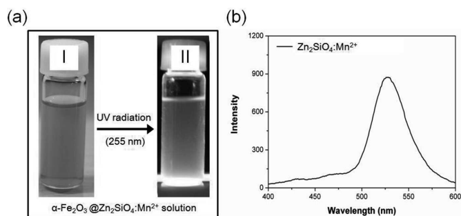
Fig. 5. (a) Photograph of solution of \alpha - \text{Fe}_2\text{O}_3@Zn_2\text{SiO}_4:\text{Mn}^{2+} in ethanol (insert; (I) no excitation, (II) excited by UV light at 255 nm). (b) Photoluminescence spectra of \text{Zn}_2\text{SiO}_4:\text{Mn}^{2+} phosphor
