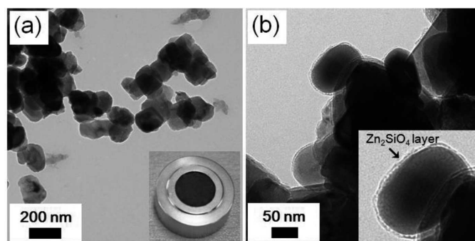
Fig. 3. TEM images of \alpha\text{-Fe}_2\text{O}_3@Zn_2\text{SiO}_4:\text{Mn}^{2+} (a) low magnification (insert image; photograph of zinc silicate-coated \alpha\text{-Fe}_2\text{O}_3 powder) (b) high magnification (insert image; The zinc silicate layer confirmed by expanded TEM image)
