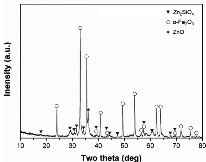
Fig. 4. XRD patterns of \text{Zn}_2\text{SiO}_4 -coated \alpha\text{-Fe}_2\text{O}_3 were calcined at 1000^\circ\text{C}
