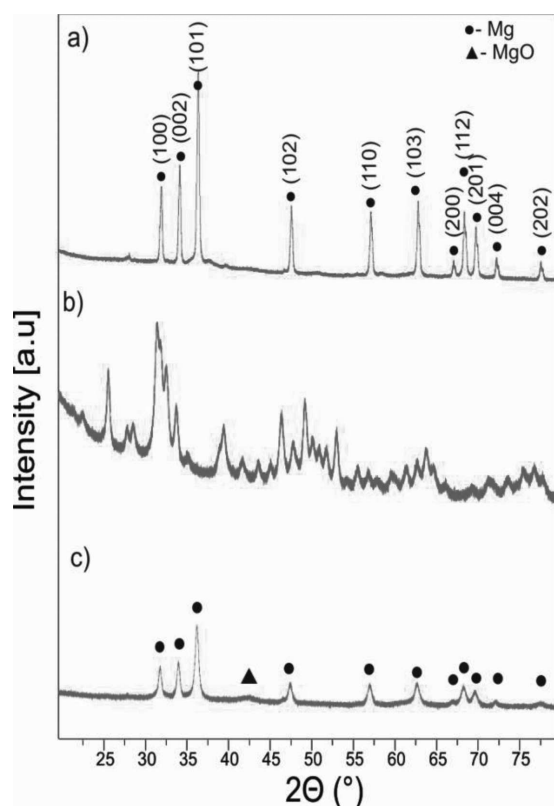
Fig. 1. XRD patterns of: a) initial Mg powder, b) initial HA powder, c) Mg-10 wt.% HA biocomposite after the 20 h MA process
