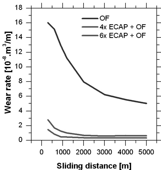
Fig. 20. The wear rate of studied materials
