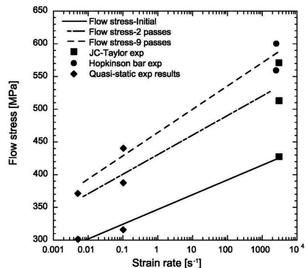
Fig. 4. Strain-rate dependence of Cu flow stress [39]
