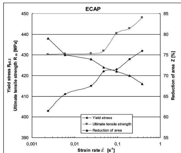
Fig. 7. The mechanical properties dependence on strain rate for ECAP samples
