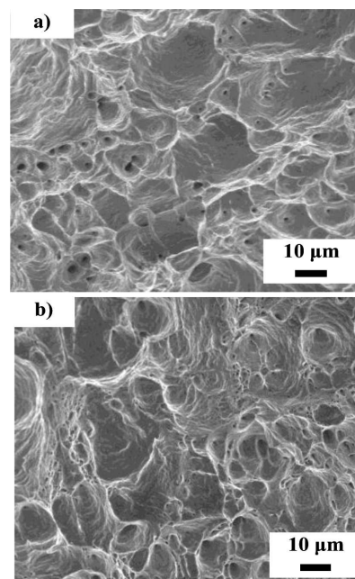
Fig. 14. SEM images of a) drawn b) ECAP samples after static tensile tests ( \dot{\epsilon} \sim 10^{-3} \text{ s}^{-1} )
