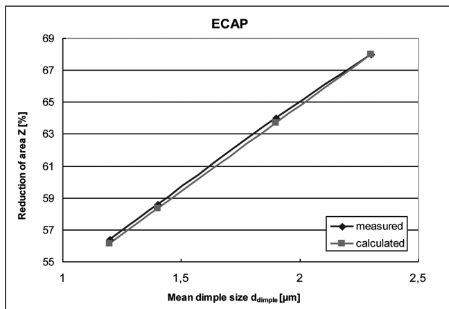
Fig. 18. Measured and calculated data of reduction of area and mean dimple size
