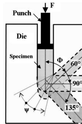
Fig. 1. Schematic illustration of ECAP equipment [18]
