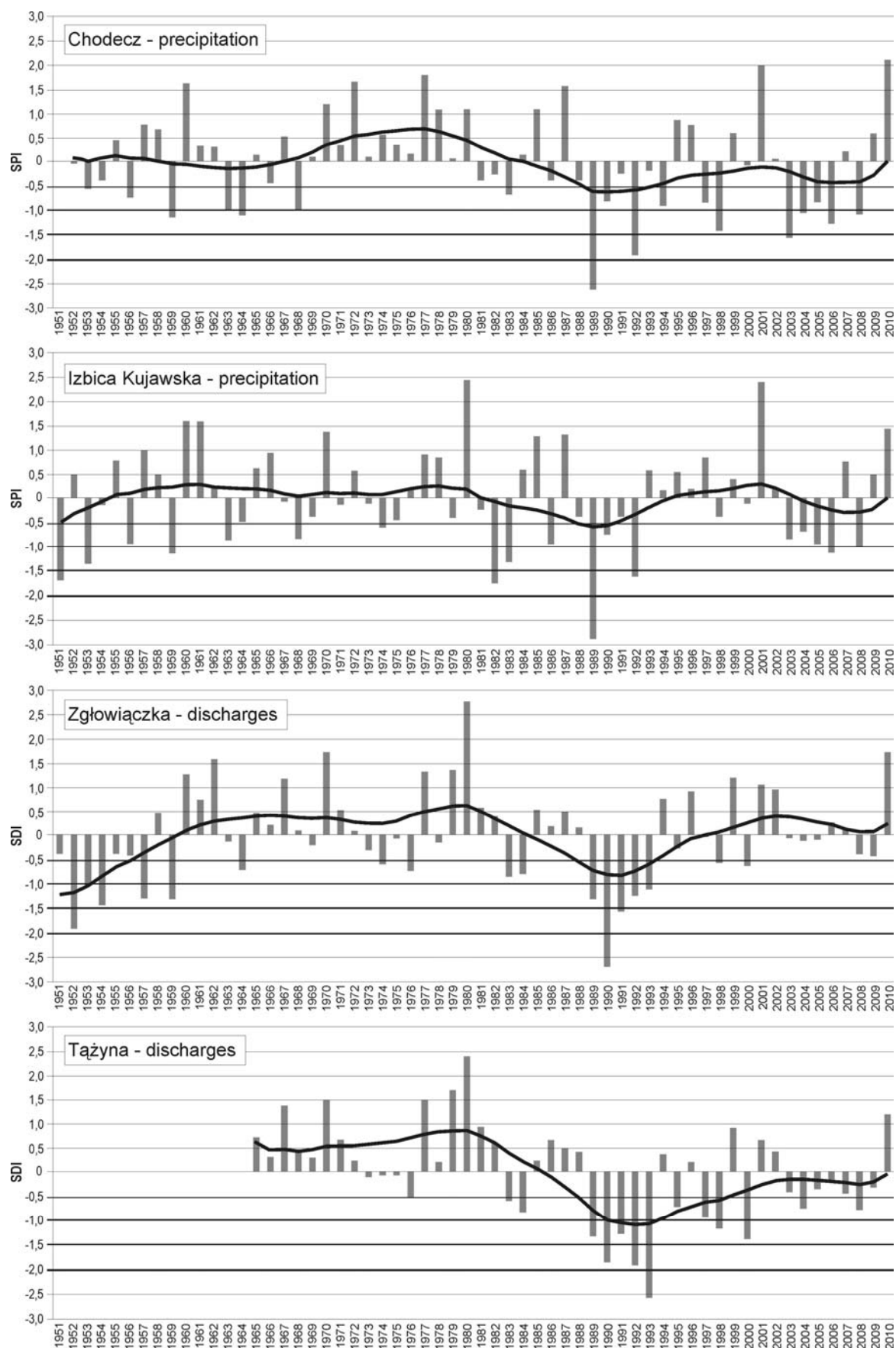
Fig. 4. Values of SPI (Standardised Precipitation Index) and SDI (Standardised Discharge Index) and their trends at selected precipitation stations and water gauges in the growing period 1951–2010; source: own elaboration
