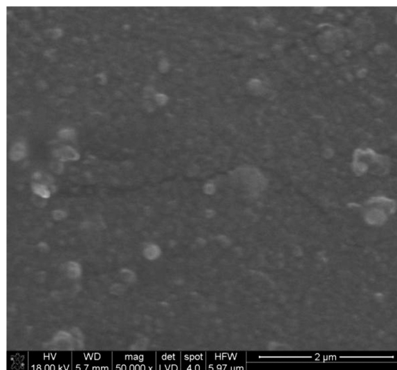
Fig. 2. Surface of \text{Al}_2\text{O}_3 -C layer on quartz glass. Layer was synthesized at 900^\circ\text{C} . Synthesis time: about 20 min
