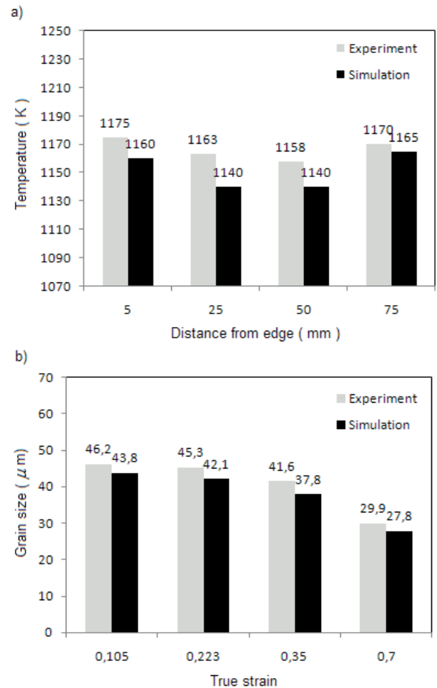
Fig. 10. Comparisons between the experimental and simulated results after cogging process in special tri-radial anvils: (a) temperature of the longitudinal section ( l_w = 0,75 ; \mathcal{E}_h = 0,70 ), (b) average grain sizes in the centre of the specimens deformed at different true strain
