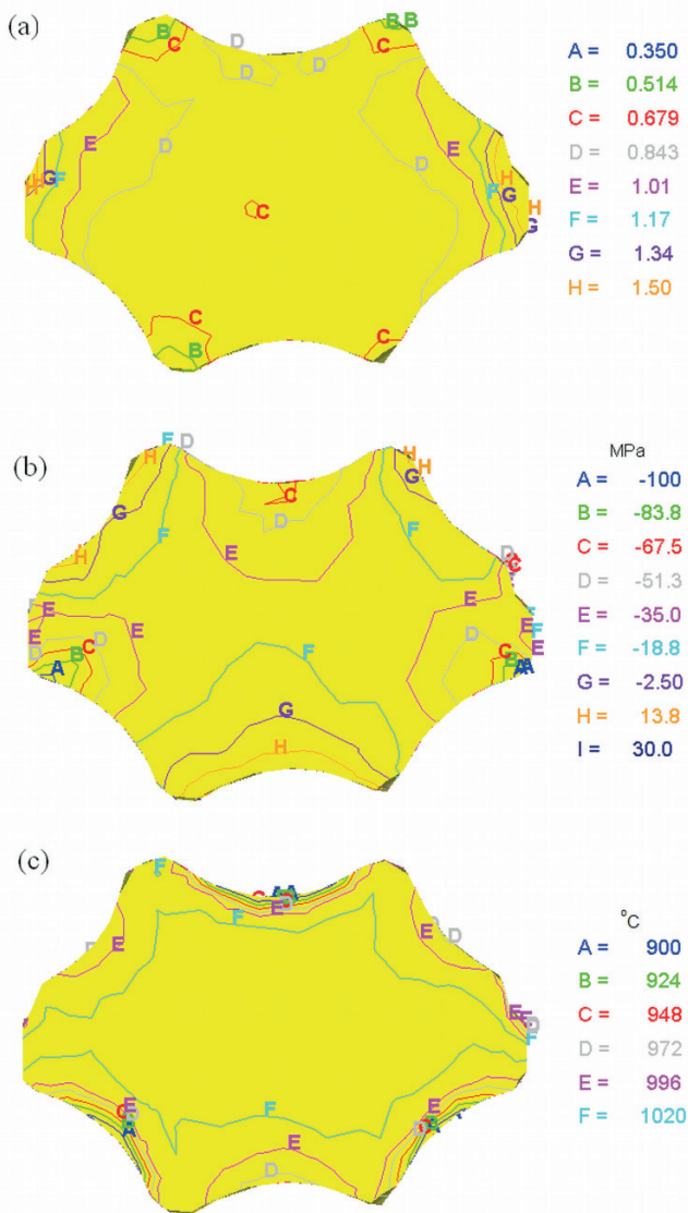
Fig. 5. Distribution of effective strain (a), mean stress (b) and temperature (c) on the specimen cross-sectional surface after cogging process in special tri-radial anvils. True strain \bar{\varepsilon}_h = 0.70
