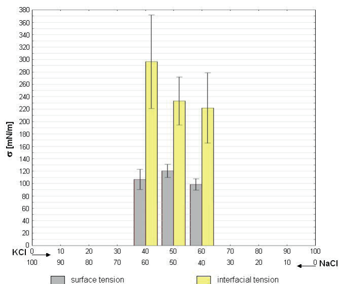
Fig.1. The measured interfacial tension values of molten salt (KCl+NaCl) mixtures of different composition fractions
