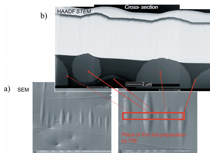
Fig. 4. Microstructure characterization of an as deposited coating; a). image obtained using SEM technique; b). image obtained by TEM technique in STEM mode [8]
