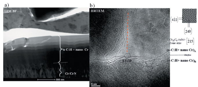
Fig. 8. Microstructure characterization of the amorphous carbon part of the coating after ball-on-disc wear test; a). TEM BF image; b). HRTEM image [8]
