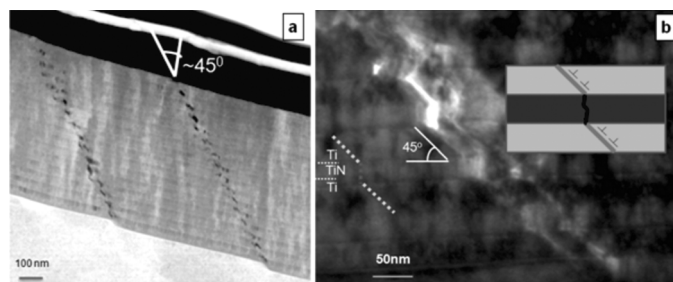
Fig. 1. Cross section TEM image of a 16 bilayer multilayer coating with modulation ratio TiN:T = 1:1; a). overview (STEM image) and b). detail of deformation mechanisms (schematics of deformation and cracking) (TEM BF image) [7]
