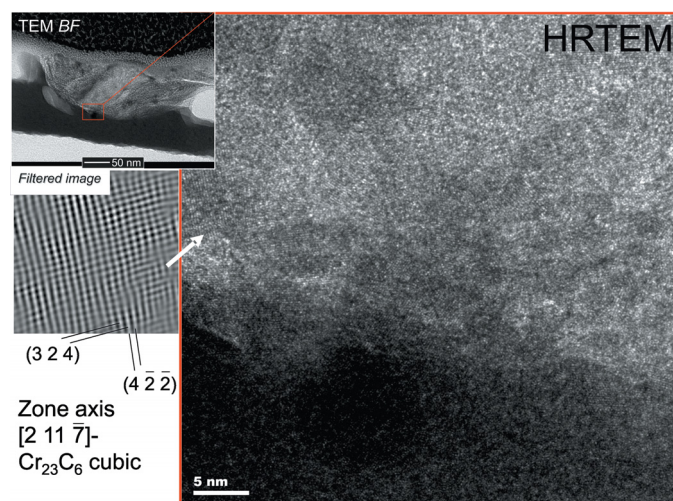
Fig. 13. HRTEM characterization of the tribofilm
