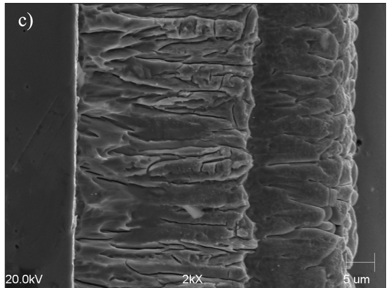
Fig. 8. (Zn) – coating, a) the Zn – segregation across the coating sub-layers; EDS analysis after initial etching, c) coating morphology after deep etching; SEM analysis
