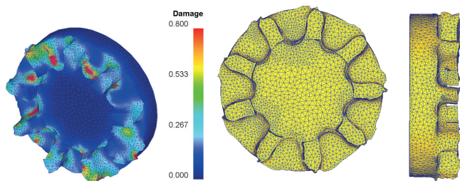
Fig. 6. Distribution of Cockcroft- Latham damage criterion (left side) and final shape of calculated head tothing (right side)
