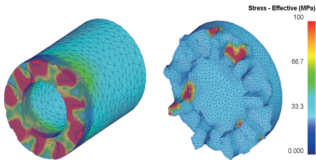
Figure 4. The shape progression of workpiece during head tothing forming with the marked distributions of effective stresses with process advancement (10% left side and 100% right side)
