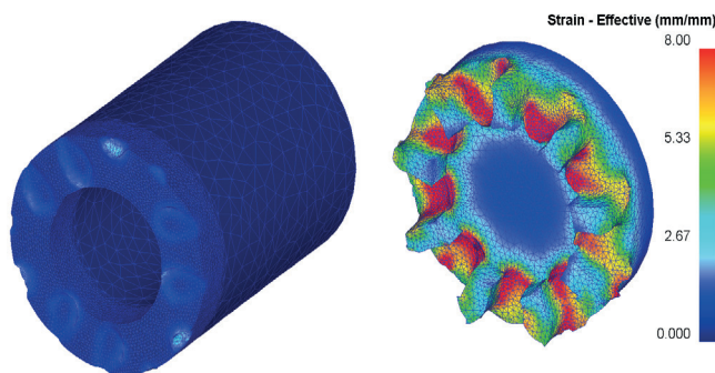
Fig. 5. The shape progression of workpiece during CWR process with the marked distributions of effective strain with process advancement (10% left side and 100% right side)
