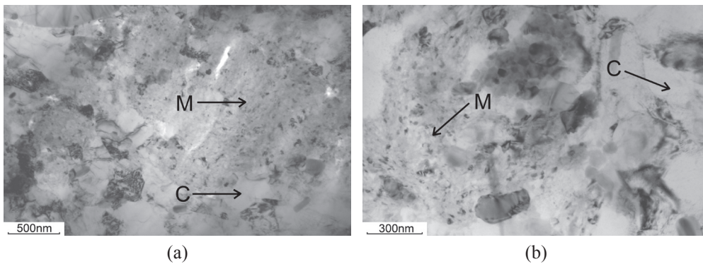
Fig. 4. TEM microstructure of MA/PM-processed and hot-extruded 2024 alloy received after a milling time of: a) 8 hours; b) 30 hours (C – chip residue, M – heavy refined microstructure)
