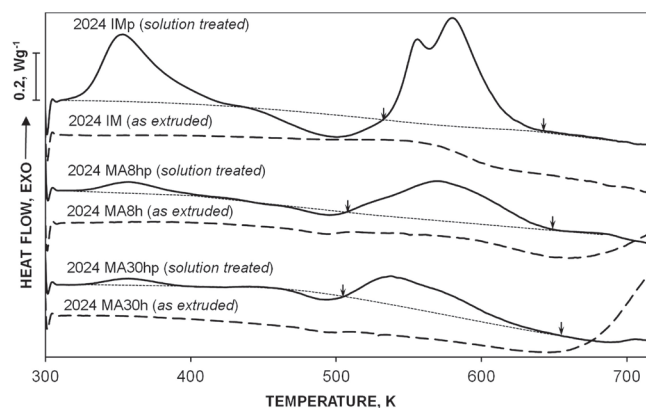
Fig. 1. DSC curves for both as-extruded and solution-treated IM and MA samples. The values of the released heat, DH, which correspond to \theta''+S'' precipitation peaks, are listed in Table 3
