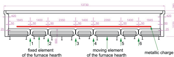
Fig. 3. Schema of walking beam furnace, the cross section
