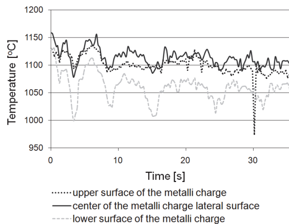
Fig. 2. Temperature change on the feedstock length after the heating process in a walking beam furnace
