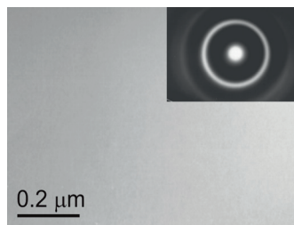
Fig. 2. TEM, with electron diffraction; Amorphous structure of samples in as quenched state
