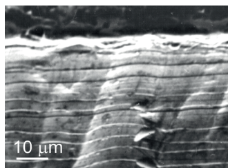
Fig. 3. SEM image of fracture morphology on the external side of tapes after decohesion in tensile test. Areas of narrow shear bands parallel to the fracture are observed near the fracture
