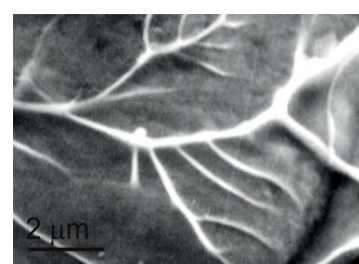
Fig. 7. SEM image of fracture surface of sample - tape. Vein-like morphology
