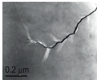
Fig. 9. TEM micrograph around a crack and at its neighbourhood. The crack front with contrast changes of amorphous structure
