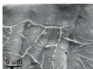
Fig. 6. SEM image of fracture surface of sample - tape. From the one edge of the smooth area fracture passes to the vein pattern area
