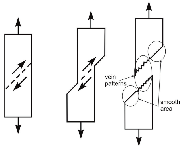
Fig. 1. The flow and fracture process by which metallic-glass samples tested in tension have fracture surfaces with two distinct areas: smooth and veined (circled). At the two ends of the shear offset the surface is smooth and shiny, suggesting that the temperature has not been very high. In the middle are the typical vein patterns, indicating the high local temperature that has been reached during fracture [16]
