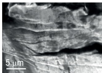
Fig. 5. SEM image of fracture morphology on the external side of tapes after decohesion in tensile test
