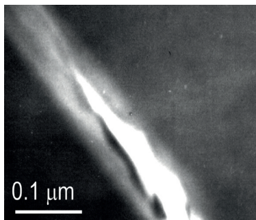
Fig. 10. TEM micrograph around a crack and at its neighbourhood. The crack front with contrast changes of amorphous structure
