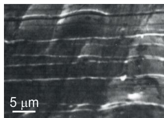
Fig. 4. SEM image of fragment of fracture morphology presented in Fig. 3. The shear bands areas and areas of wedge-shaped zones connecting bands are visible
