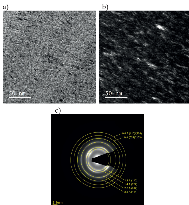
Fig. 3. Structure of the AlCrSiN coating: a) TEM bright-field image, b) TEM dark field image, c) corresponding SAED pattern
