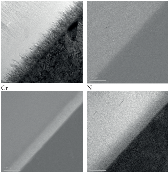
Fig. 9. Structural EFTEM images with elemental sensitivity obtained for transition zones existing in AlCrSiN coatings formed on the X40CrMoV5-1 steel substrate
