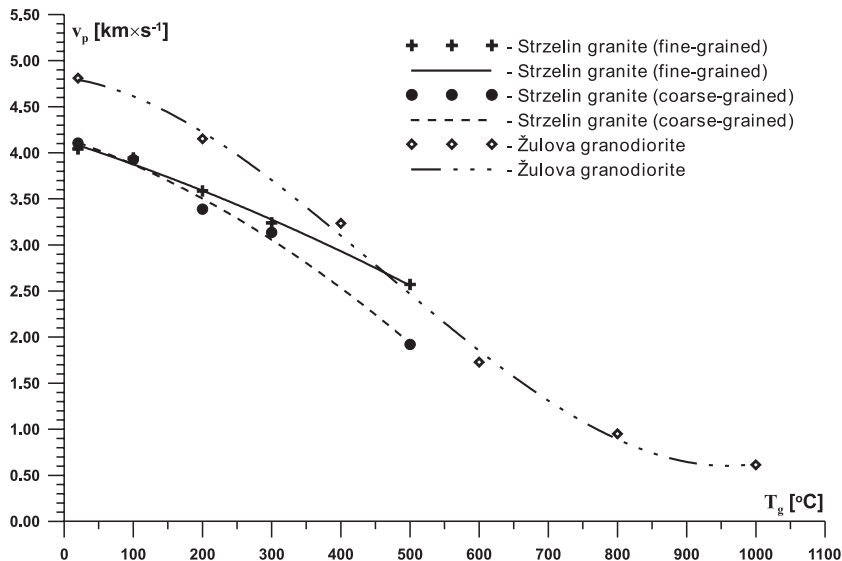
Fig. 7. Comparison of the results of studies into the relationship between the primary wave velocity and the heating temperature for the Strzelin granites and the Żulova granodiorite; the granodiorite part after Kožušnikova (1999)
