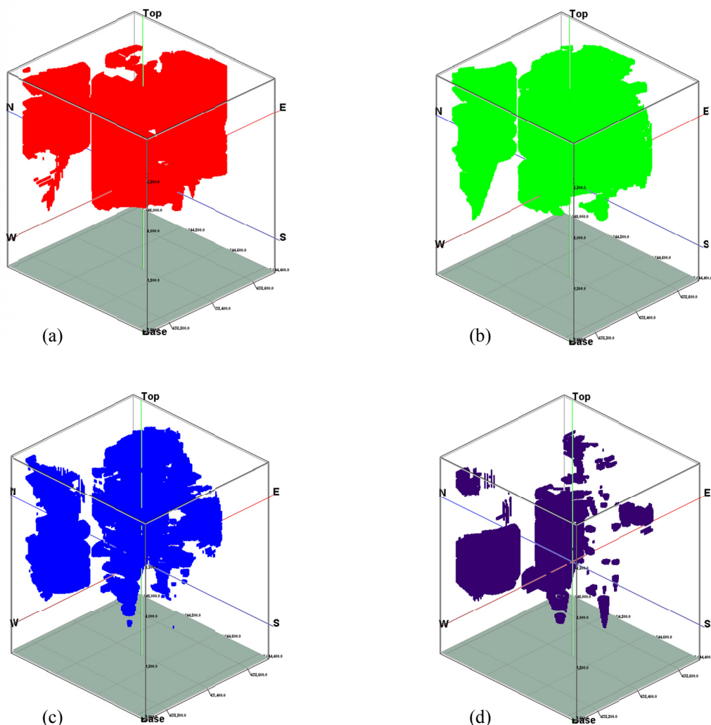
Fig. 7. RQD populations in the Kahang deposit based on thresholds defined from the RQD-N fractal model (a) very poor zones; (b) very poor & poor zones; (c) fair and good zones; (d) excellent zones
