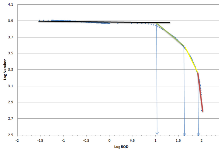
Fig. 6. RQD-N log-log plot in the Kahang deposit
