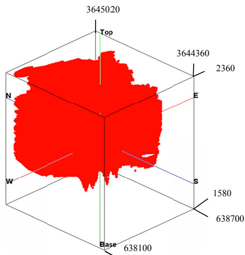
Fig. 3. Porphyric quartz diorite unit within the deposit
