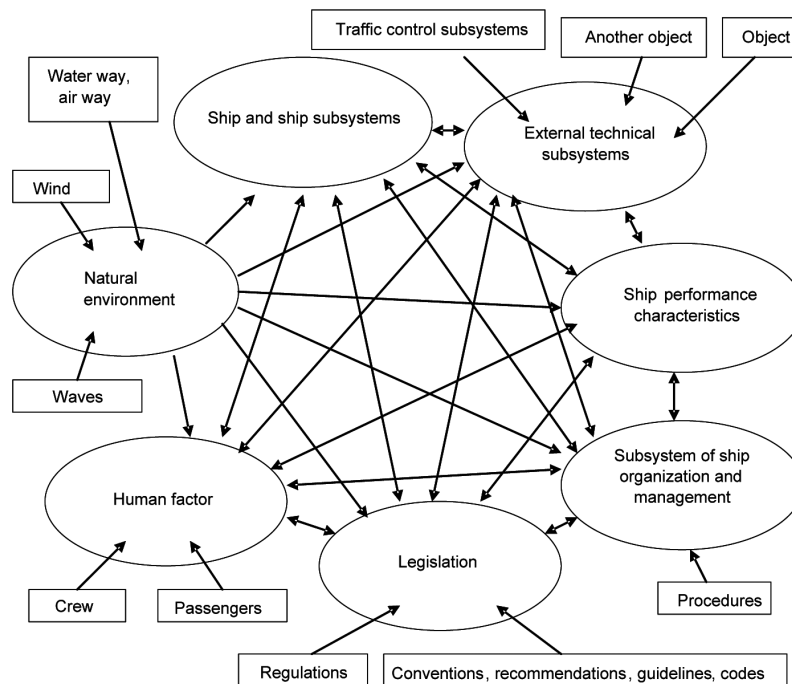
Fig. 2. The structure of interrelations existing between the data elements of the safety system of complex technical object including an aircraft or ship
