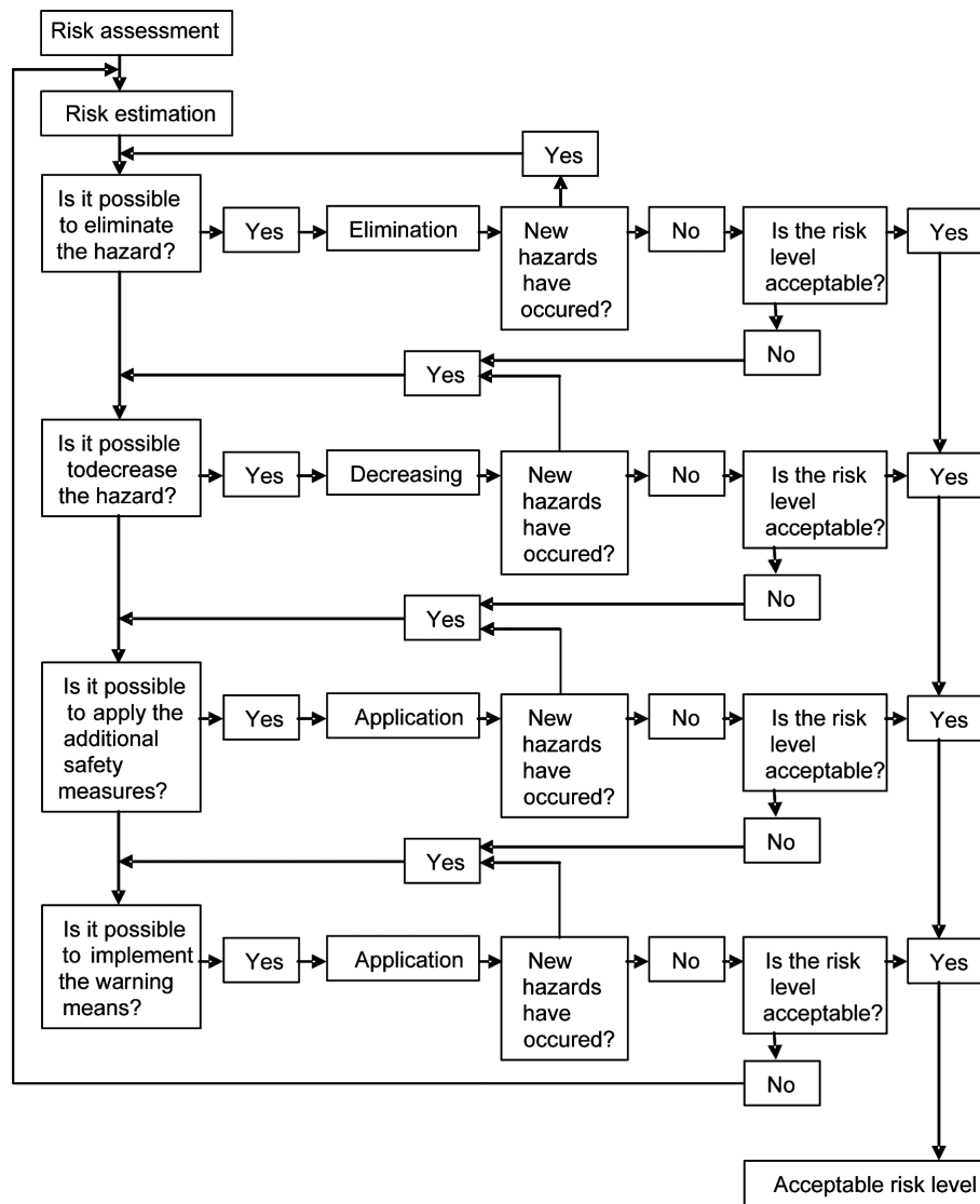
Fig. 5. The structure of the safety management system of the complex technical objects concerning the application in the waterborne and airborne transportation
