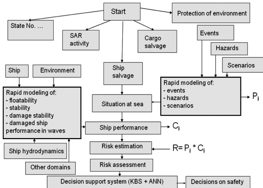
Fig. 6. The structure of the object in damaged conditions safety system which enables the risk and safety assessment during a catastrophe at sea
