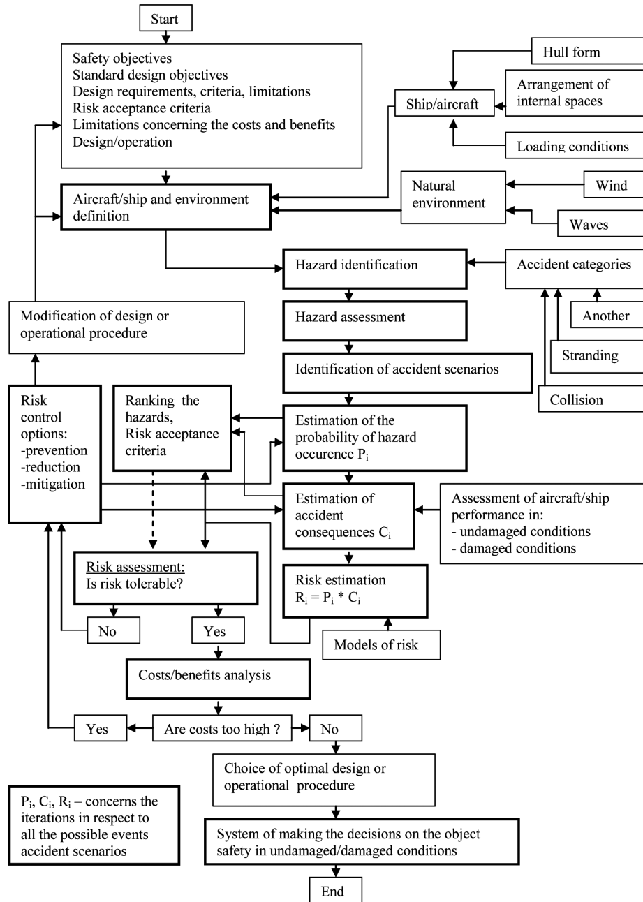
Fig. 4. The structure of the proposed method of safety assessment of complex technical objects which is based on the performance assessment and risk assessment
