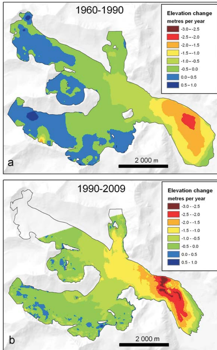
Fig. 4. Mean annual elevation change ( dh/dt ) of Hørbyebreen for the period 1960–1990 (a), with an up-build visible in the upper zones and the period 1990–2009 (b), with thinning over the entire glacier area.
