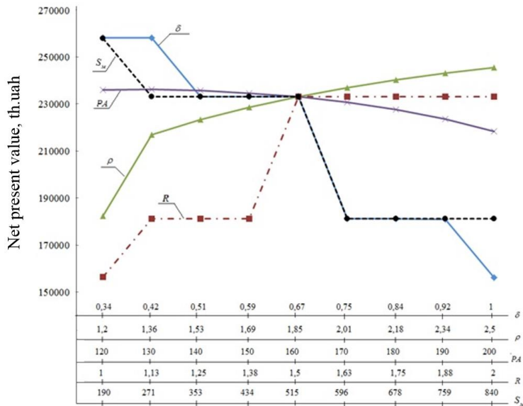
Fig. 8. Investment performance of logistics system functioning dependence on different cities parameters: \delta – irregularity factor; \rho – density of retailers location; PA – automobiliation level; R – nonlinearity factor; S_m – city area.
