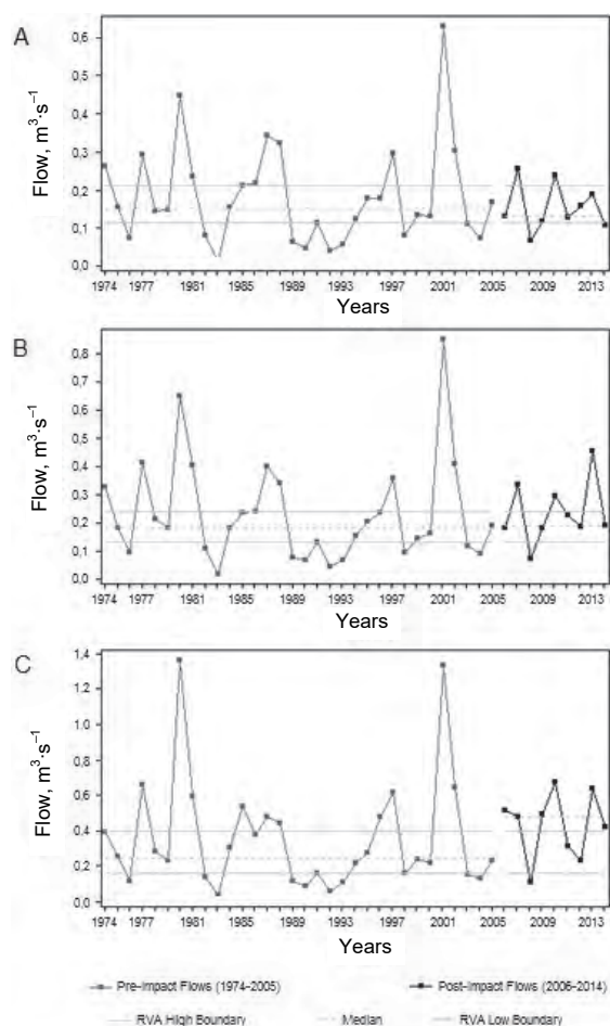
Fig. 4. The impact of the Stare Miasto reservoir on magnitude and duration of annual extreme water conditions: 7-day minimum (A), 30-day minimum (B), 90-day minimum (C); RVA as in Fig. 3; source: own study
