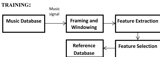
Fig. 1. Training phase.
