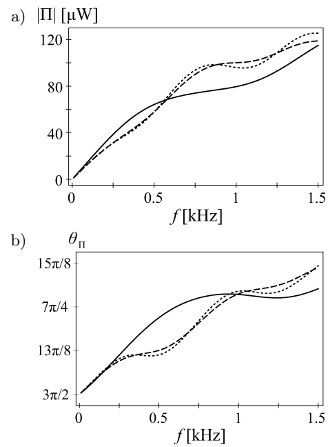
Fig. 11. Sound power: a) modulus |\Pi| , b) phase \theta_{\Pi} as the functions of the vibration frequency for \varphi_0 = 5\pi/4 . The line keys: solid – the piston's location I and M_{ap} = 16 , dashed – the piston's location II and M_{ap} = 28 , and dotted – the piston's location III and M_{ap} = 18 .
