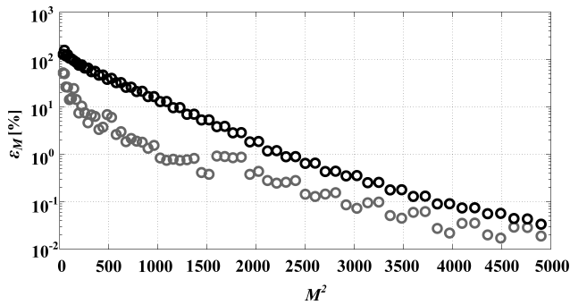
Fig. 17. Convergence error rate (log scale) of radiation efficiency with discretization of the hemispherical surface parameter M^2 : Mode by Mode —, in frequency bands - - .
