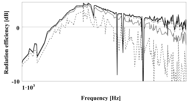
Fig. 7. Radiation efficiency calculated for several values of radius of the hemisphere: 2 m —, 5 m — — —, 10 m — · — · —, 20 m — — — —, 30 m · · · ·, 60 m — — — — (Detail of Fig.6).
