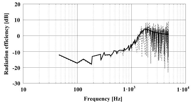
Fig. 9. Radiation efficiency calculated for several values of the parameter M : M' = 10 (dotted line), M' = 20 (solid line), M' = 50 (dashed line).
