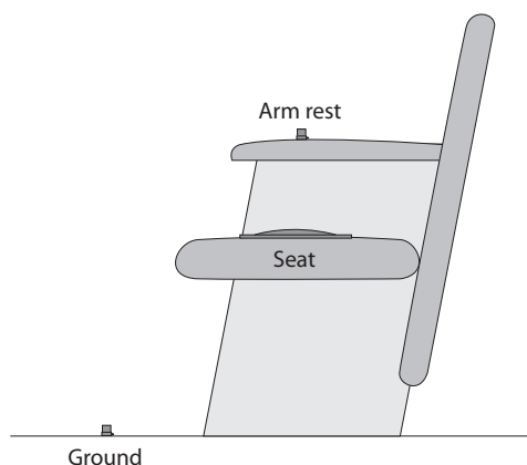
Fig. 4. Measurement setup with accelerometers on the ground, the seat and the arm rest.
