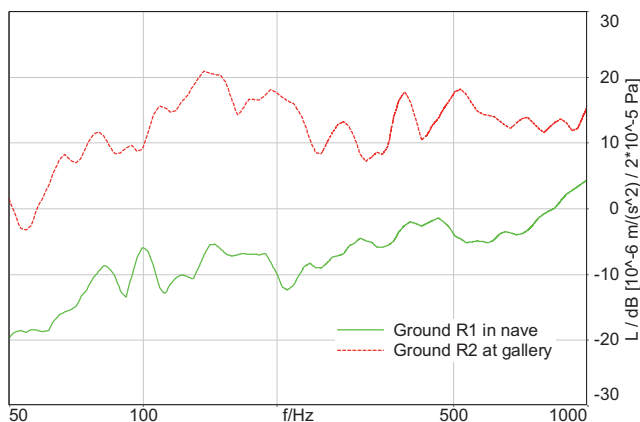
Fig. 11. Transfer functions (FFT 65536, 1/24th octave intensity averaging) between acceleration on the ground and the sound pressure at ear height in the nave and in the gallery.
