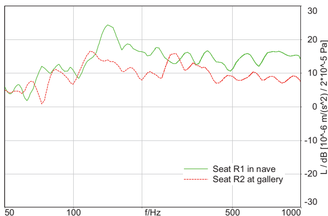
Fig. 13. Transfer functions (FFT 65536, 1/24th octave intensity averaging) between acceleration at the seat and the sound pressure at ear height in the nave and in the gallery.
