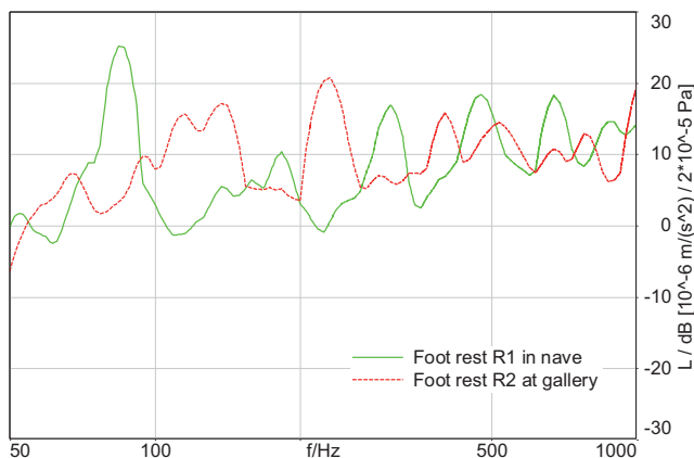
Fig. 12. Transfer functions (FFT 65536, 1/24th octave intensity averaging) between acceleration at the feet and sound pressure at ear height in the nave and in the gallery.
