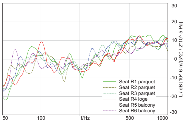
Fig. 6. Transfer functions (FFT 65536, 1/24th octave intensity averaging) between acceleration on the seat and the sound pressure at ear height at all receiver positions.
