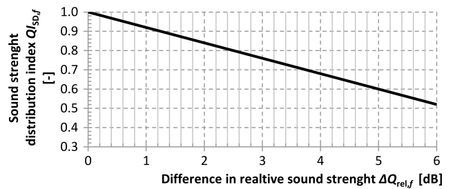
Fig. 7. Relationship between difference in relative sound strength \Delta G_{rel,f} and the value of sound level distribution index QI_{SD,f} for a given frequency.
