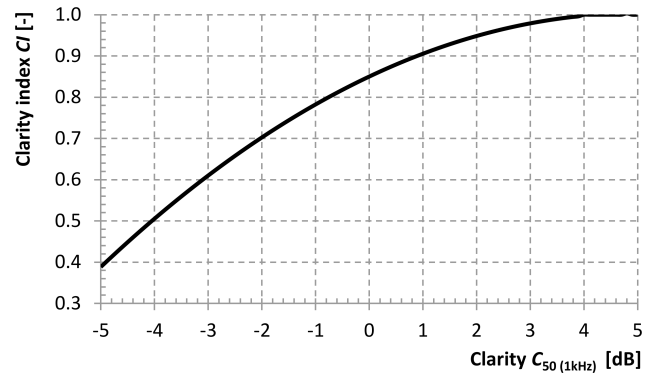
Fig. 5. Relationship between the clarity C_{50(1\text{kHz})} and the auxiliary clarity index CI .
