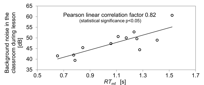
Fig. 1. Relationship between reverberation time RT_{mf} and the level of background noise during lessons (MIKULSKI, RADOSZ, 2012), where RT_{mf} is the arithmetic mean of the reverberation time from 500 Hz, 1000 Hz and 2000 Hz octave bands.
