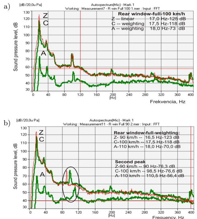
Fig. 3. Comparison of energies using Z -, C - and A -weighting of the same acoustic signal at different car speeds: a) 100 km/h; b) different speeds.
