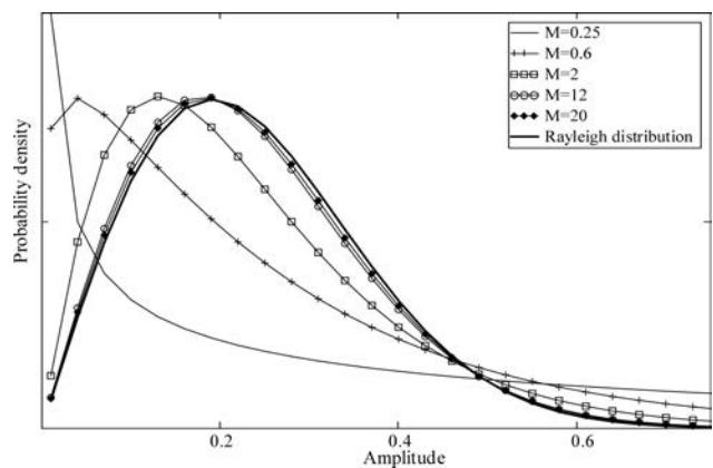
Fig. 1. Plots of the K -distribution pdf for various values of the effective number of scatterers.
