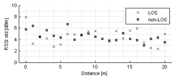
Fig. 5. Standard deviation of measured RSSI (LOS and non-LOS).
