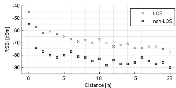
Fig. 4. Median of measured RSSI (LOS and non-LOS).
