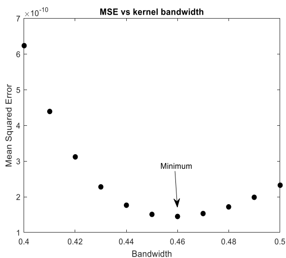
Fig. 8. MSE vs kernel bandwidth for 2.4 GHz.
