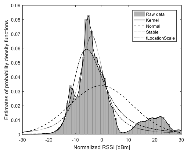
Fig. 9. PDF estimates for 2.4 GHz band (WLAN ch. 14).
