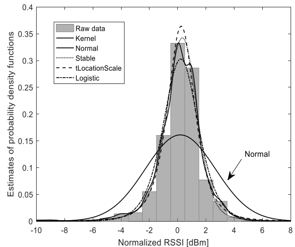
Fig. 3. PDF estimates for 868 MHz band.
