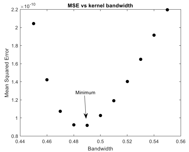
Fig. 12. MSE vs kernel bandwidth for 5 GHz.
