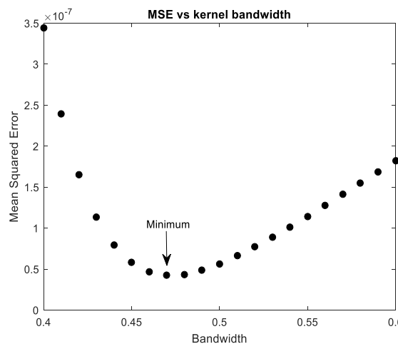
Fig. 6. MSE vs kernel bandwidth for 2.4 GHz.
