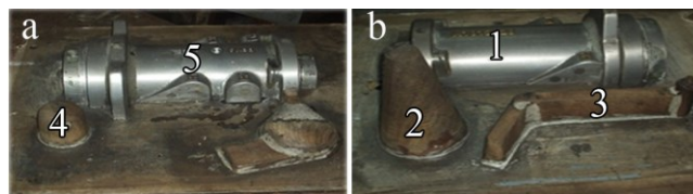
Fig. 7a. Drag pattern. 7b. Cope pattern
