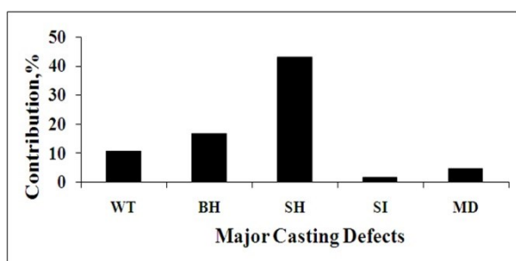
Fig. 2. Bar chart of casting defects
