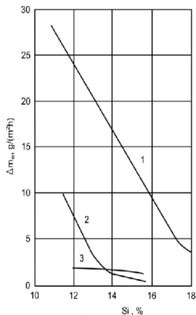
Fig. 1. Corrosion rates of high silicon cast irons as a function of silicon content and corrosive media. 1 – 35 % HCl solution, temp. 80°C, 2 – 40 % H 2 SO 4 solution, temp. 60°C, 3 – 20 % HNO 3 solution, temp. 60°C [5]
