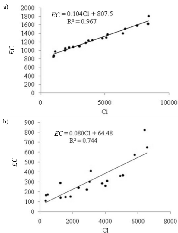
Fig. 7. Regression analysis of \text{Cl}/\text{EC} during: (a) November 2013, (b) April 2014; source: own study
