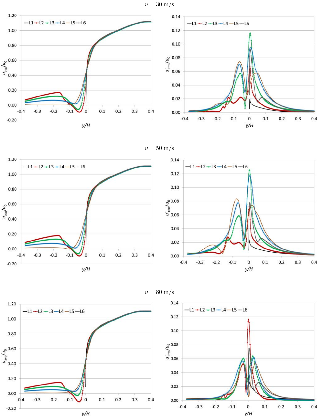
Fig. 10. Value of the flow normalised mean velocity and the RMS value of fluctuations in the velocity horizontal component for the free flow velocity values of u = 30, 50 and 80 m/s.
