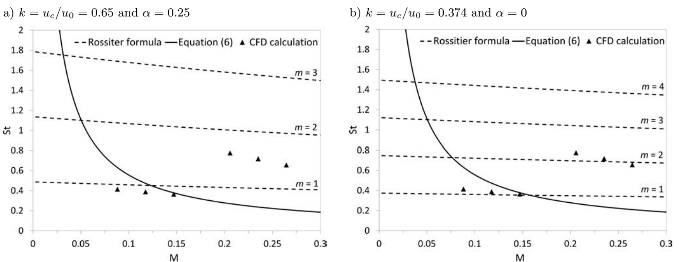
Fig. 9. Strouhal number depending on the Mach number – comparison between empirical relations and numerical calculations for: a) parameters assumed following by ROSSITER (1964) and WITTICH (2011), b) parameters from calculations and HASSAN et al. (2007).
