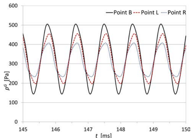
Fig. 5. Gauge pressure fluctuations at the channel flow velocity of 50 m/s.
