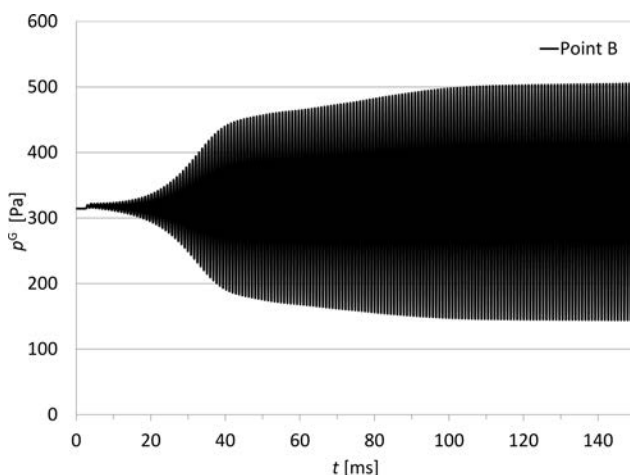
Fig. 5. Gauge pressure fluctuations at the channel flow velocity of 50 m/s.
