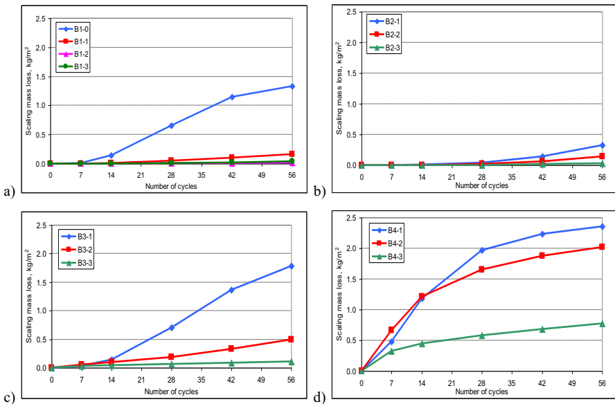
Fig. 1. Scaling mass loss – mean values
